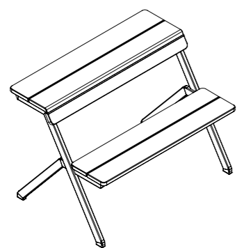
ISOMETRIC
